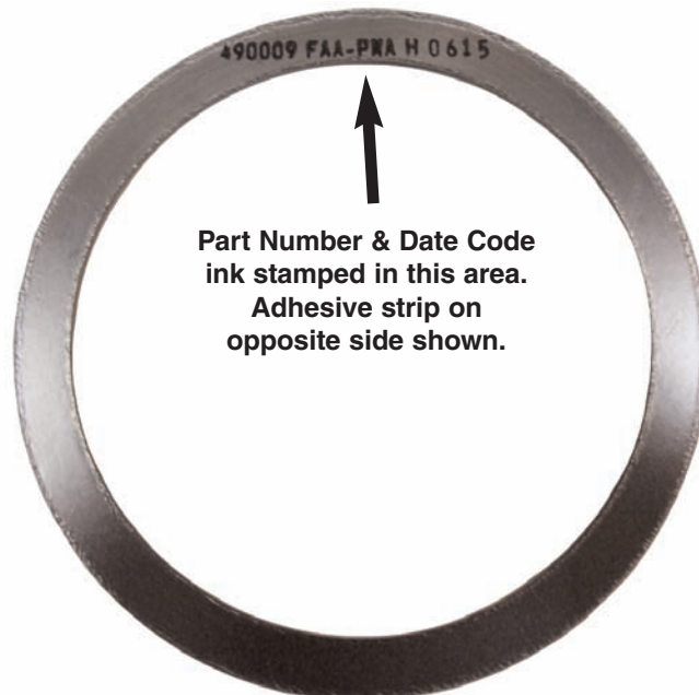
Figure 1 - P/N CF600400-00 Turbine Housing Gasket (Superseded by HET P/N 490009 Turbine Housing Gasket)
