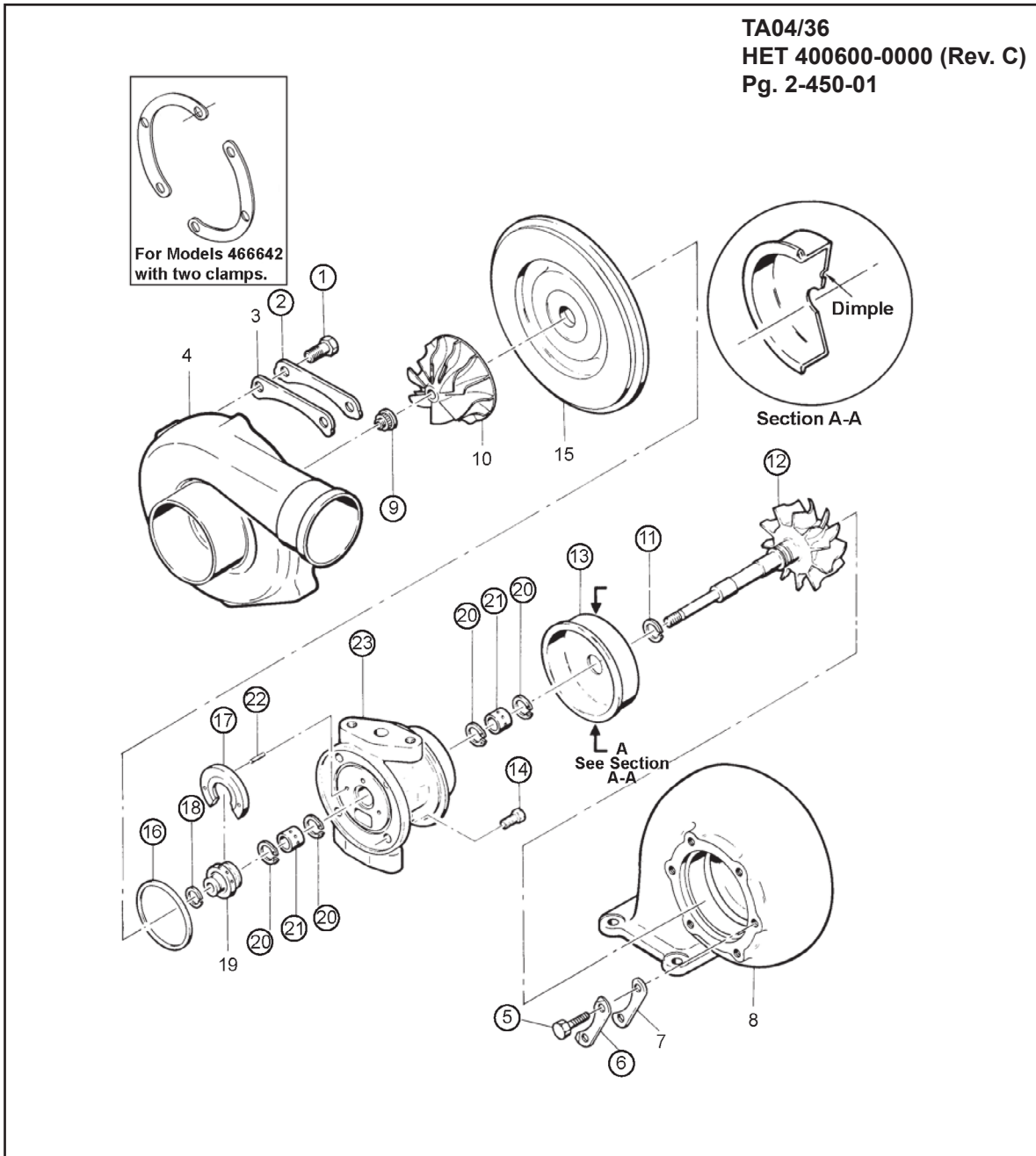
Turbine Wheel Assembly (Itm# 12) and Compressor Wheel Nut (Itm# 9) Figure 1.1
