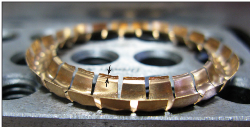
Figure 3 - Raised Material on Inside Diameter (may or may not be present)
