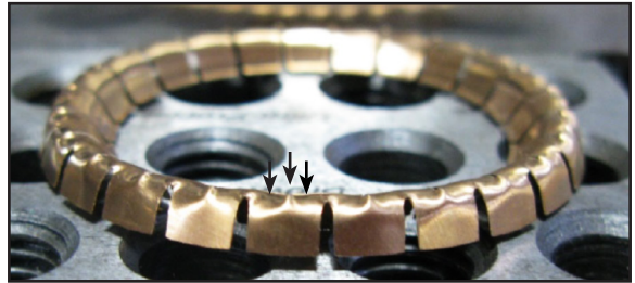
Figure 2A - Rigid Lower Bend Radius
