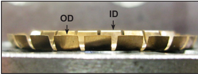
Figure 1 - Outside Diameter Lower than Inside Diameter.
